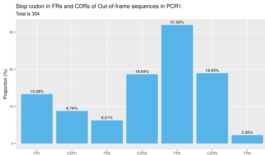
Figure 11: Proportion of stop codons in any given CDR or FR of out-of-frame sequences in PCR1 The percentages show the frequency of stop codons in a given region relative to the total number of stop codons present.
