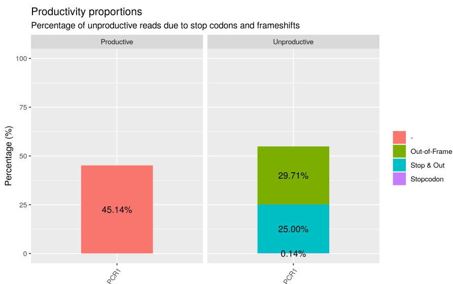
Figure 9: Productivity rate of sequences in PCR1
