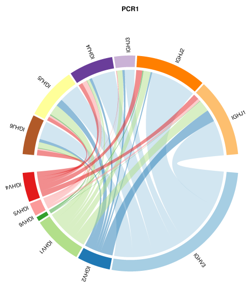
Figure 7: V family germline distribution in PCR1 The percentage of IGHV families after germline annotation using IgBLAST.
