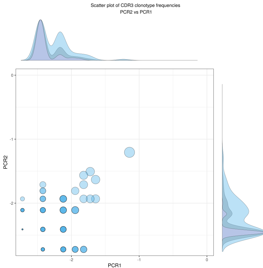
Figure 22: Log-scaled scatter plot of clonotype frequencies in PCR1 and PCR2 Point size denotes mean frequency of the 2 samples and marginal density plots are colour coded by overlapping (blue), non-overlapping (purple), and all (grey) clonotypes.
